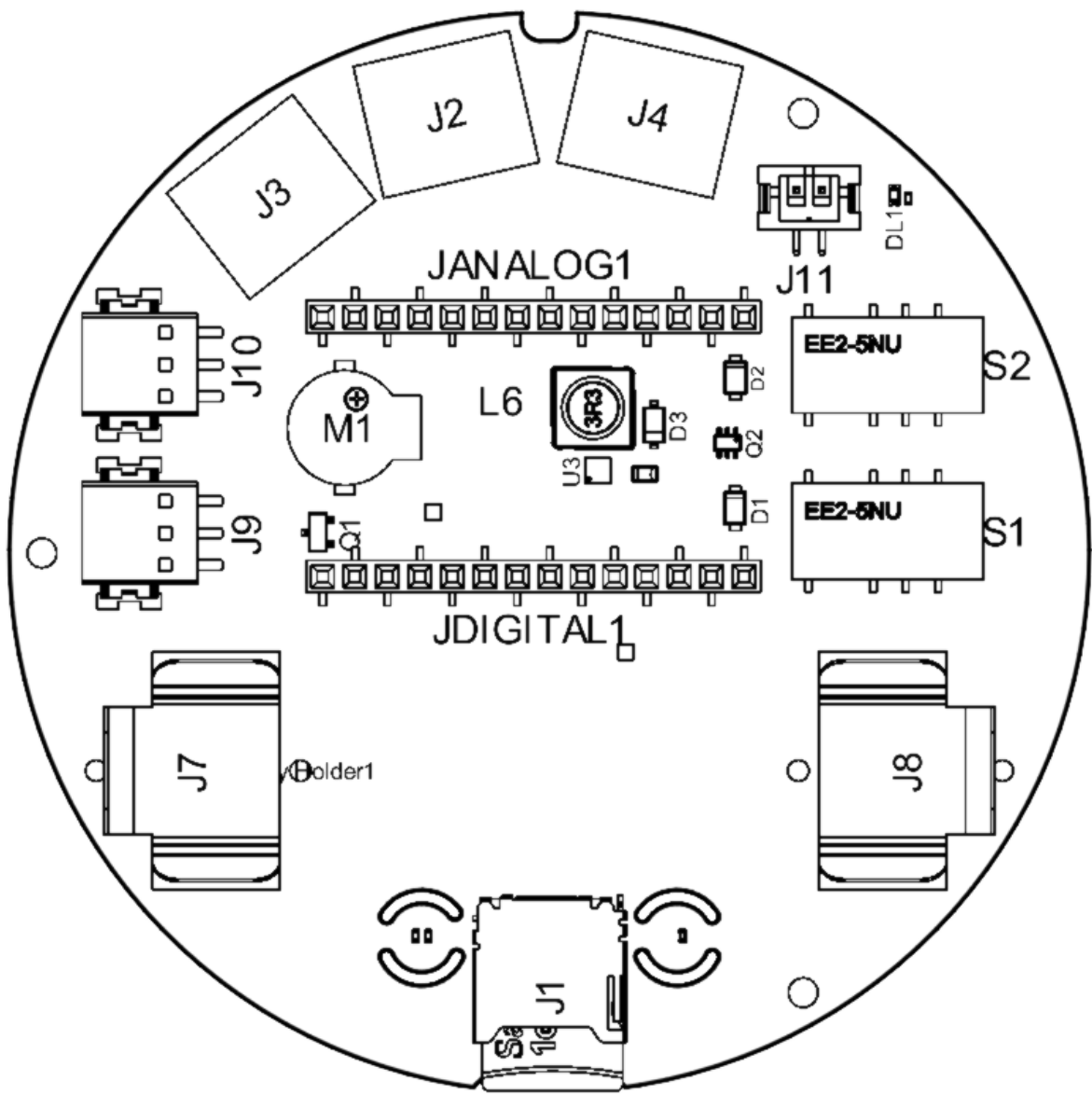
Bottom view
